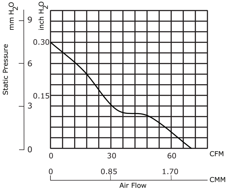
CFM-9225V-242-440
