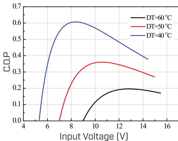
COP Vs. Input Voltage, V ( \Delta T = 40\sim 60\text{ °C} )
