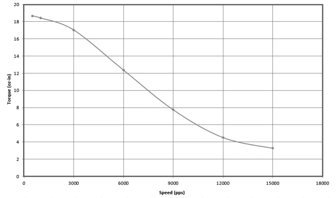
Same Sky P/N NEMA11-20-01D-AMT112S Lin Engineering P/N WO-211-20-01 (1.8 Step Motor) 24 Vdc, 0.67 Amp/Phase, R208, 1/2 Stepping
