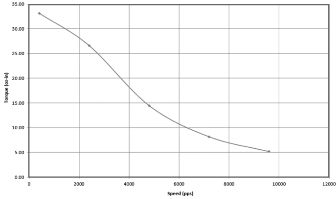
Same Sky P/N NEMA17-16-06SD-AMT112S Lin Engineering P/N WO-4118M-06S (1.8 Step Motor) 24 Vdc, 0.7 Amp/Phase, R208, 1/2 Stepping
