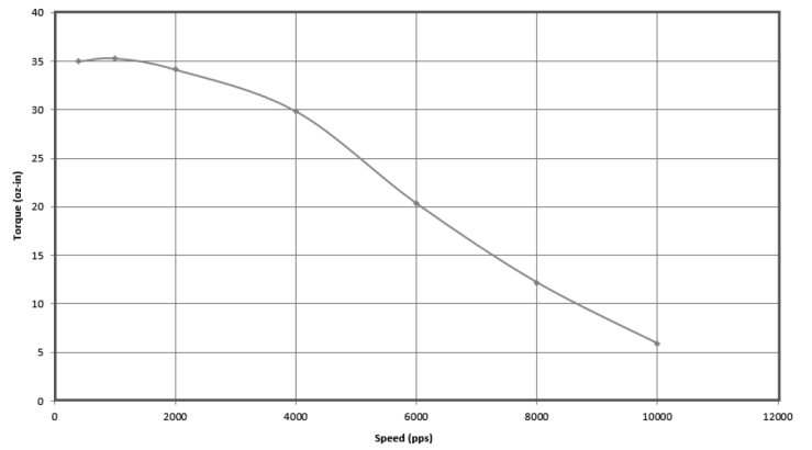
Same Sky P/N NEMA17-16-06PD-AMT112S Lin Engineering P/N WO-4118M-06P (1.8 Step Motor) 24 Vdc, 1.4 Amp/Phase, IB462, 1/2 Stepping
