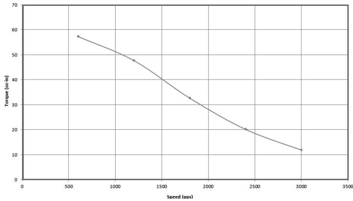
Same Sky P/N NEMA17-16-06SD-AMT112S Lin Engineering P/N WO-4118M-06S (1.8 Step Motor) 24 Vdc, 0.7 Amp/Phase, R208, 1/2 Stepping
