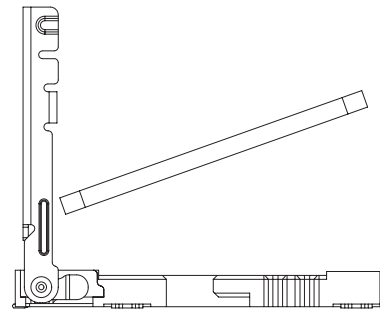
STEP 1 INSERT Nano-SIM CARD
